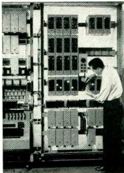
Large cabinet (left) is space-control unit, heart of Intelix system being installed by Penn. R.R. Operator receives on the teleprinter a coded message from a ticket seller for a reservation. Unit automatically selects from trays in cabinet the one containing car diagrams for trains on day requested. Operator selects proper diagram and flashes back confirmation. At right is one-sixth of the behind-the-scenes brain of the Intelix system. Gas triodes, shown at immediate left of engineer, convert incoming teleprinter characters into currents that actuate appropriate relays to bring desired tray file in front of operator at left
